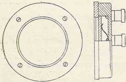
Fig. 1.—Elevation and part section of the Tungram light element.
